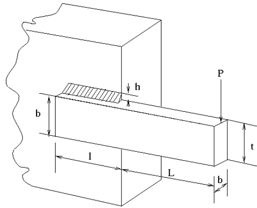
Figure 2: Welded beam
