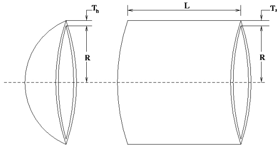
Figure 3: Pressure Vessel
